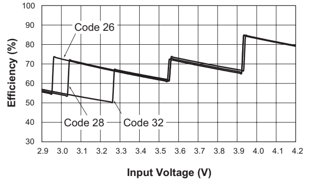
Efficiency vs. Input Voltage (D1-D2 = 3.5V, D3-D4 = 3.2V)
